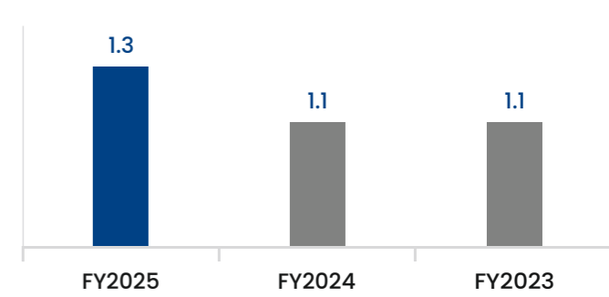
Current Ratio
